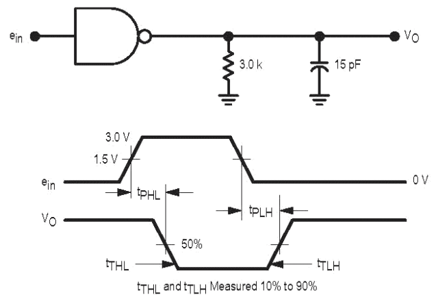
Figure 6. Switching Response
