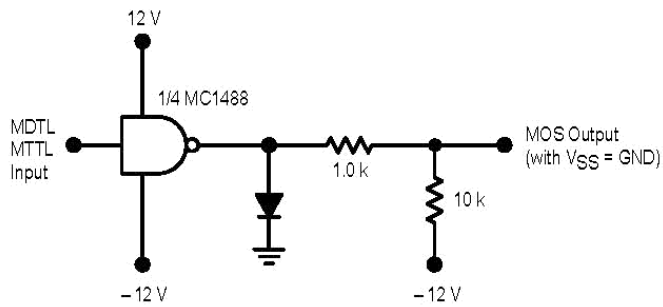
Figure 14. MDTL/MTTL – to –MOS Translator
