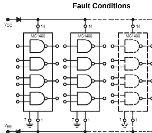
Figure 13. Power Supply Protection to Meet Power Off
