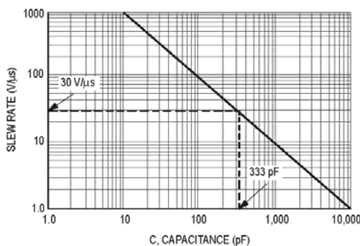
Figure 12. Slew Rate versus Capacitance for I_{SC}=10\text{mA}
