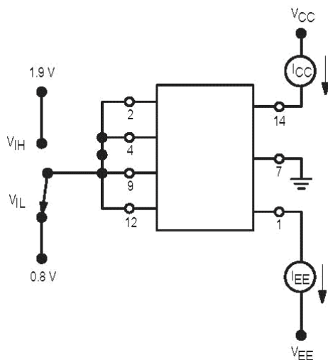
Figure 5. Power Supply Current
