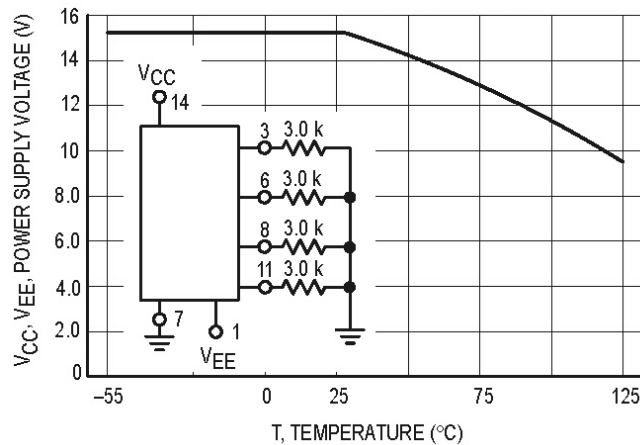
Figure 11. Maximum Operating Temperature Versus Power Supply Voltage
